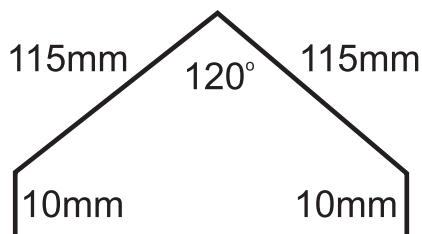
Ridge Capping
