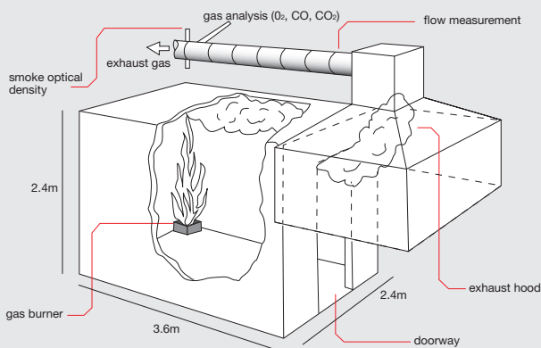
The gas burner exposes the polycarbonate sheeting to 100kw for 10 minutes, and then 300kw for a further 10 minutes until flashover is reached.
